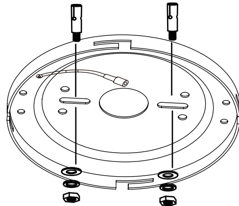
Concrete Ceiling
